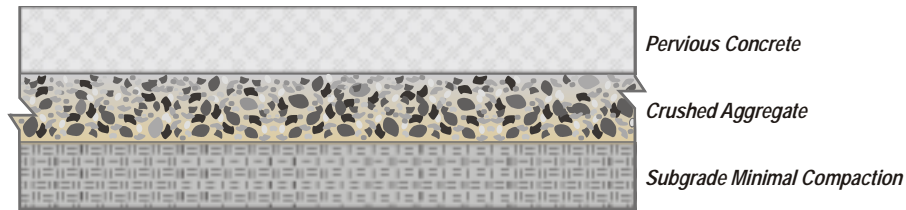
Figure 6-2 Porous Pavement
